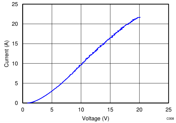
Figure 6-2. Surge Curve (tp = 8/20 μs), Pin IO to GND
