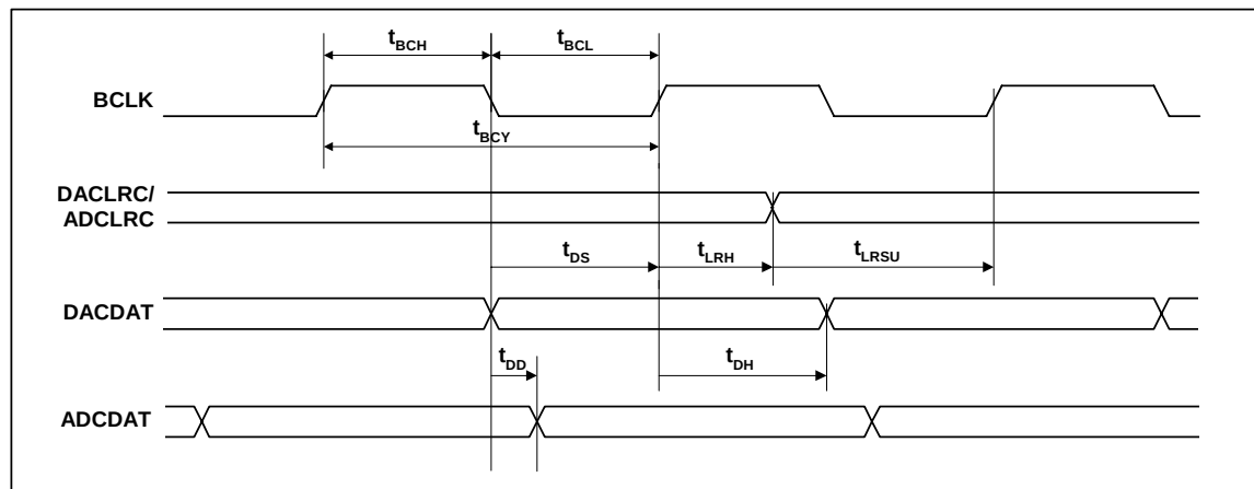
Figure 6 Digital Audio Data Timing – Slave Mode
