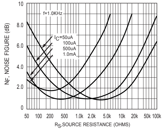
Figure 6.Source Resistance Effects
