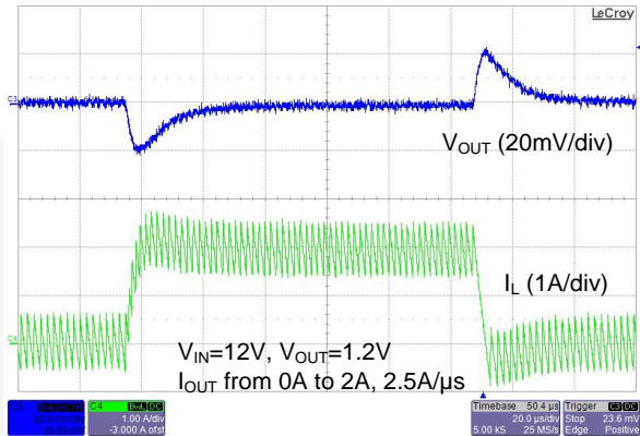
Figure 19. Load Transient from 0% to 50% Load Current
