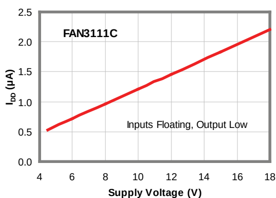
Figure 7. I_{DD} (Static) vs. Supply Voltage
