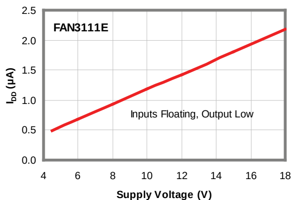
Figure 8. I_{DD} (Static) vs. Supply Voltage
