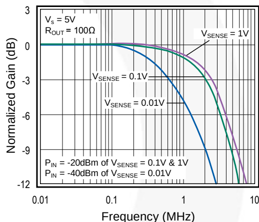
Figure 7. Frequency Response
