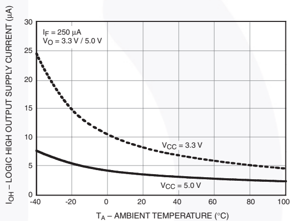
Figure 6. Logic High Output Current ( I_{OH} ) vs. Ambient Temperature
