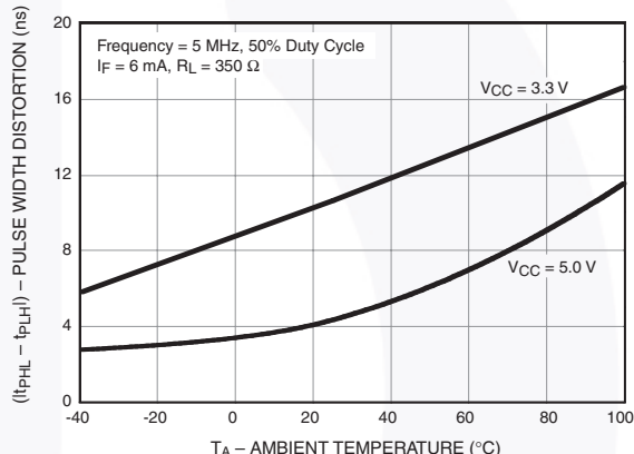
Figure 12. Pulse Width Distortion vs. Ambient Temperature
