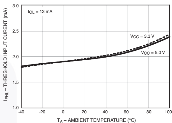
Figure 4. Threshold Input Current ( I_{FHL} ) vs. Ambient Temperature
