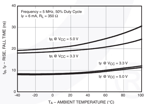
Figure 14. Rise Time ( t_R ) and Fall Time ( t_F ) vs. Ambient Temperature
