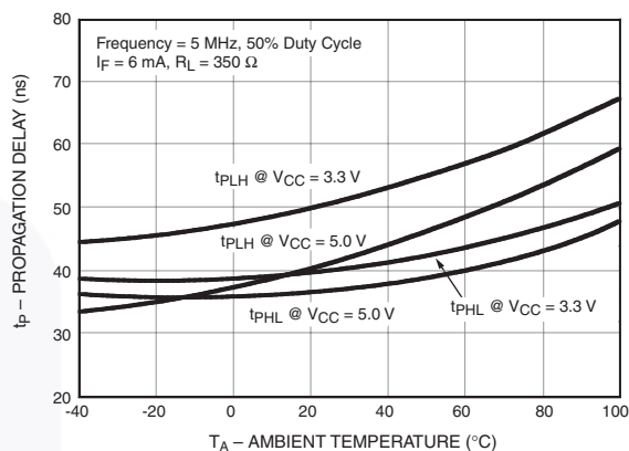
Figure 10. Propagation Delay vs. Ambient Temperature
