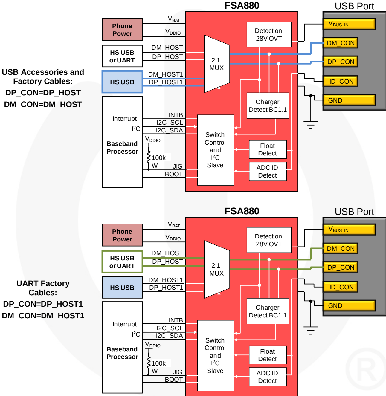
Figure 8. Switch Configurations
