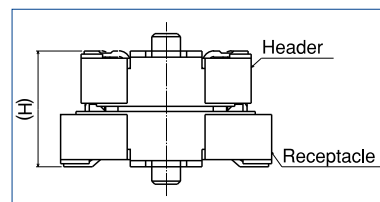
(H):Reference dimension
