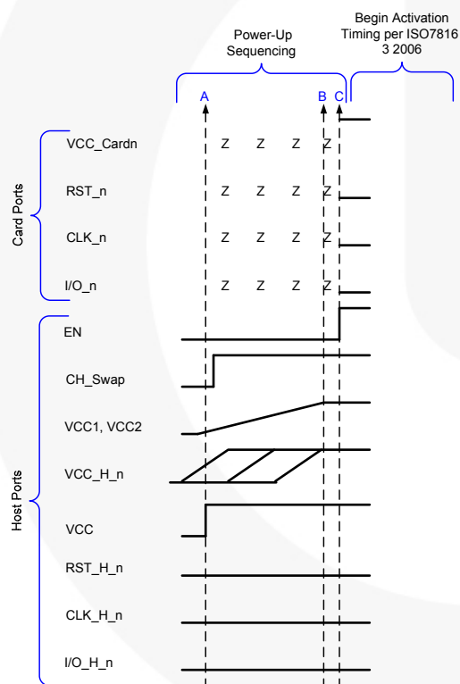
Figure 16. Power-Up Sequencing
