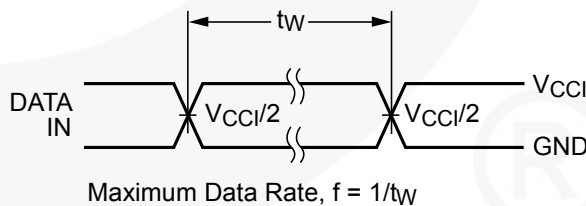
Figure 8. Maximum Data Rate
