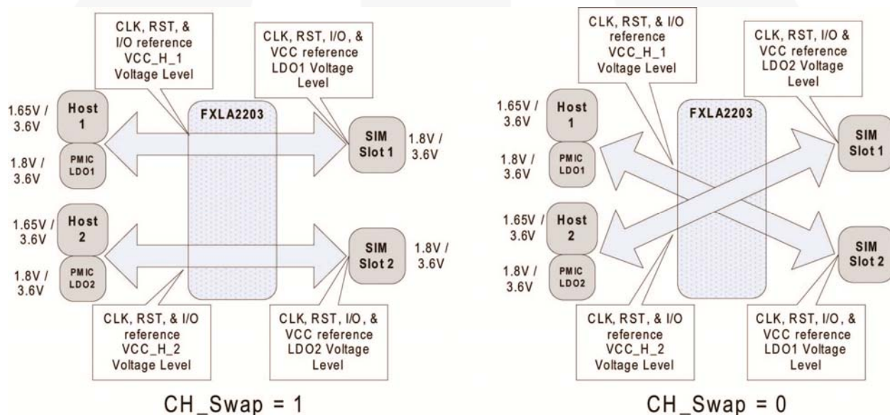
Figure 11. Voltage Translation
