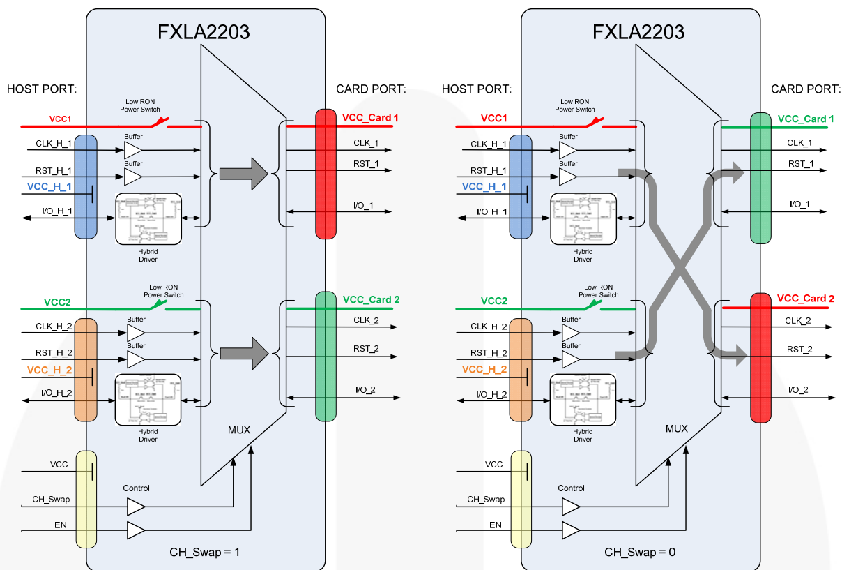
Figure 1. Block Diagram
