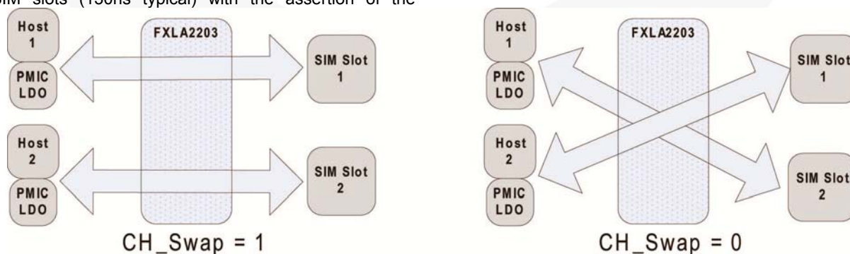
Figure 10. CH_Swap
