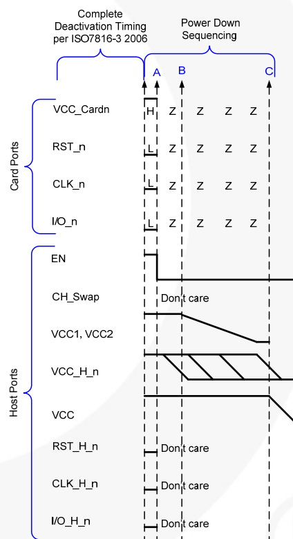
Figure 17. Power-Down Sequencing
