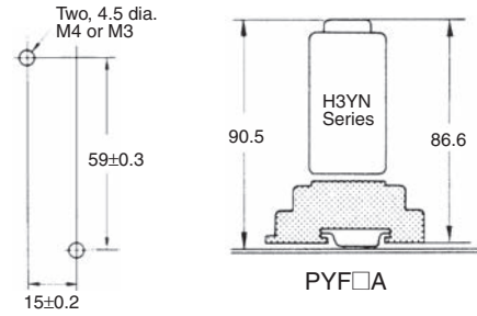
Mounting Holes
