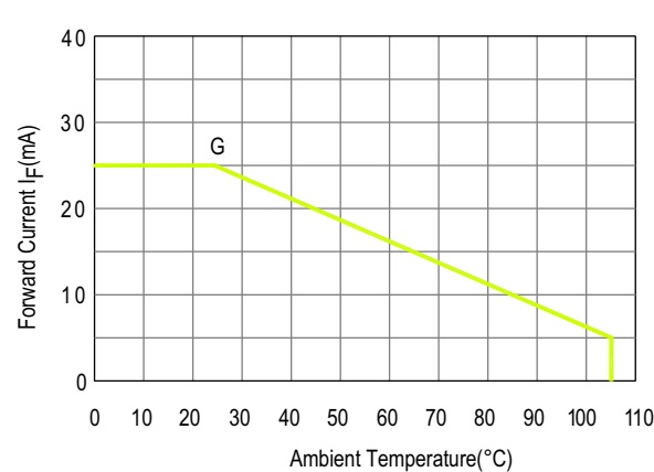
Figure 3: Allowable DC Current vs. Ambient Temperature
