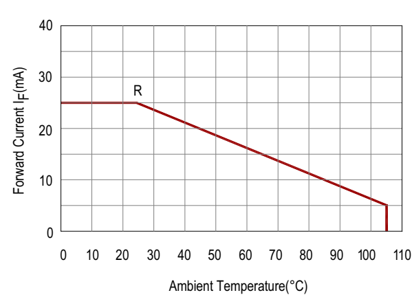
Figure 11: Allowable DC Current vs. Ambient Temperature
