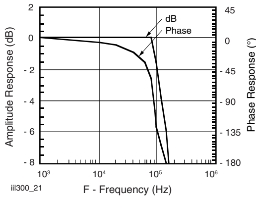
Fig. 16 - Amplitude and Phase Power Supply Control
