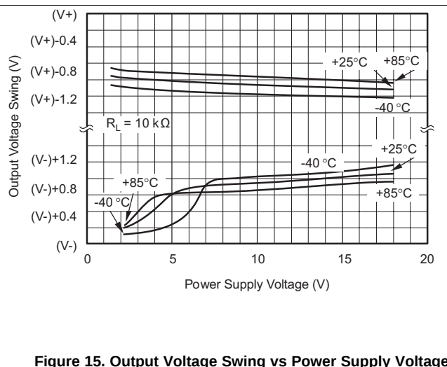
Figure 15. Output Voltage Swing vs Power Supply Voltage
