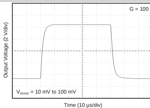
Figure 19. Step Response
