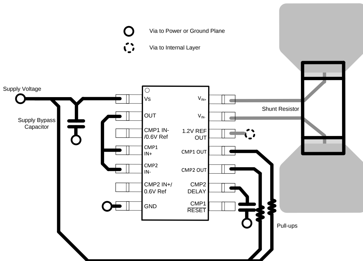
Figure 44. Layout Recommendation
