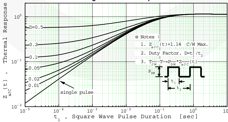
Fig 11. Thermal Response
