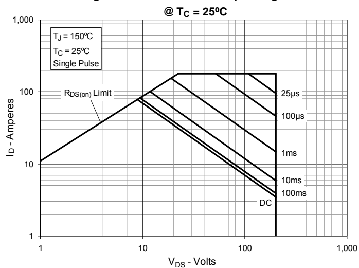
Fig. 15. Forward-Bias Safe Operating Area @ T_C = 25°C
