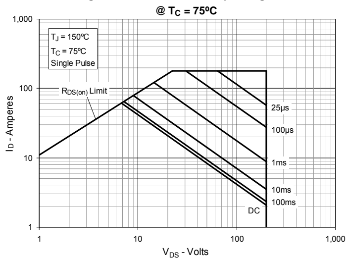
Fig. 16. Forward-Bias Safe Operating Area @ T_C = 75°C
