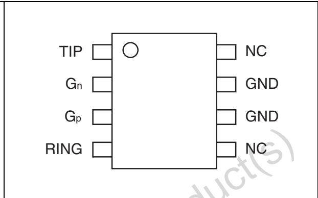
Figure 2. Pin-out configuration
