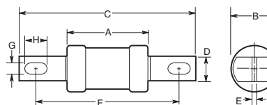
L09C/M09C/P09C (Center Blades)
