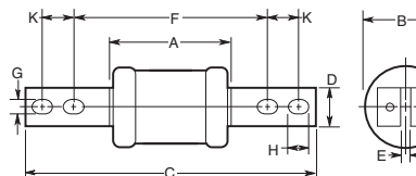
P11C/R11C (Center Blades)
