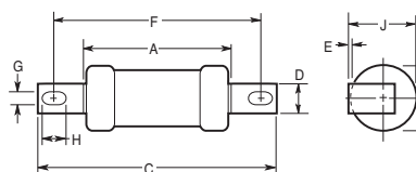
K07C/K07CR/ L14C/M14C (Offset Blades)
