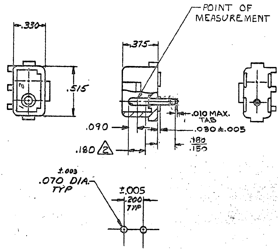
RECOMMENDED LAYOUT FOR .062 THICK P.C. BOARD
