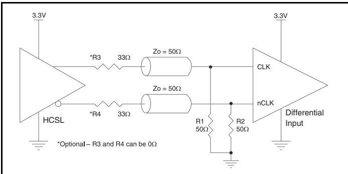
Figure 2E. HiPerClocks CLK/nCLK Input Driven by a 3.3V HCSSL Driver
