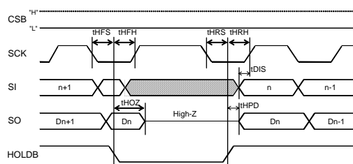
Figure 3. HOLD timing
