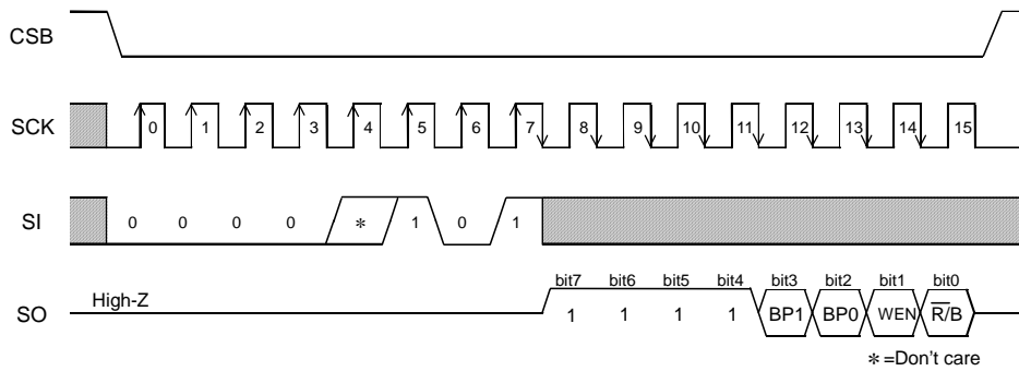
Figure 41. Status Register Read Command (BR25H010/020/040-WC)
