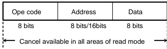
Figure .46 READ Cancel Valid Timing
