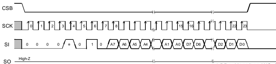
Figure 37. Write Command (BR25H010/020/040-WC)
