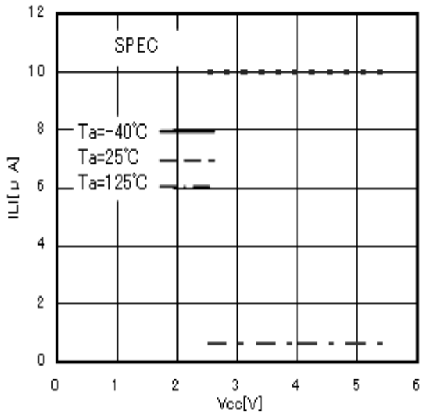
Figure 10. Input Leak Current vs Supply Voltage
