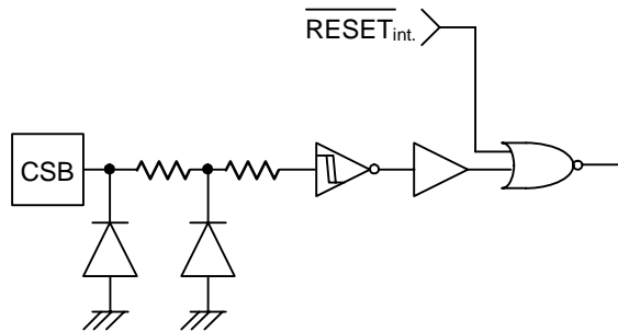
Figure 56. CSB Input Equivalent Circuit
