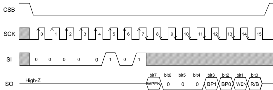
Figure 42. Status Register Read Command (BR25H080/160/320-WC)
