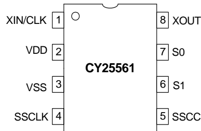
Figure 1. 8-pin SOIC pinout
