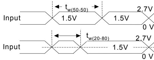
Figure 6. Voltage Waveforms—Pulse Duration [6]
