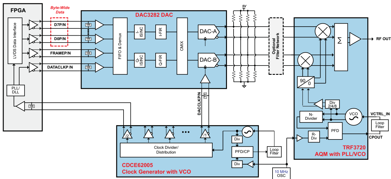
Figure 84. System Diagram of Direct Conversion Radio
