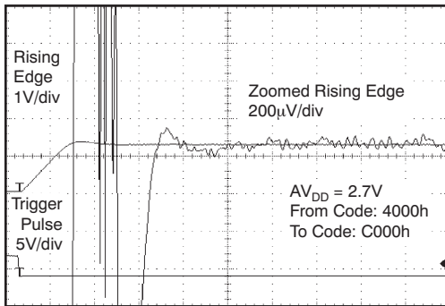
Time (2µs/div) Figure 108.
