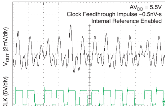
CLOCK FEEDTHROUGH 2MHz, MIDSCALE
