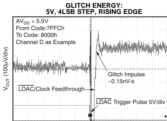
Time (5µs/div) Figure 62.
