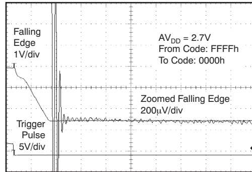
Time (2µs/div) Figure 107.
