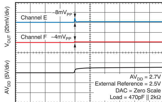
Time (4ms/div) Figure 111.
