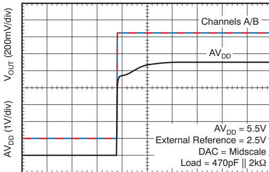
POWER-ON GLITCH RESET TO MIDSCALE
