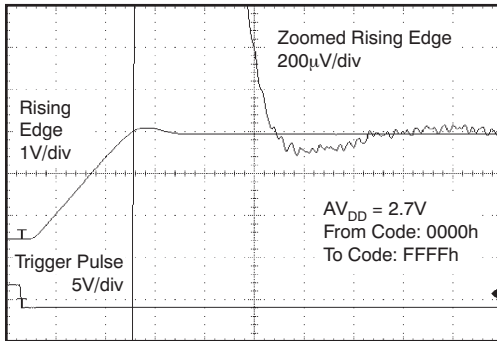
Time (2µs/div) Figure 106.
