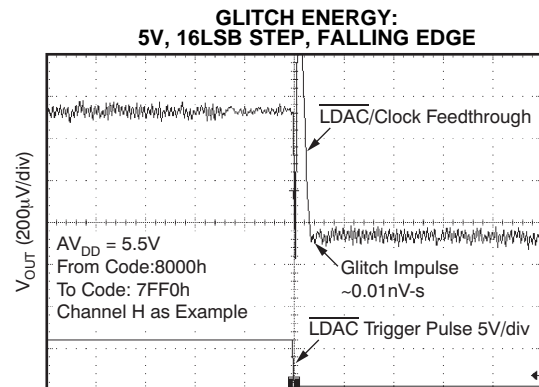
Time (5µs/div) Figure 65.
