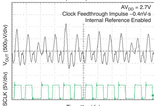
Time (1µs/div) Figure 110.
