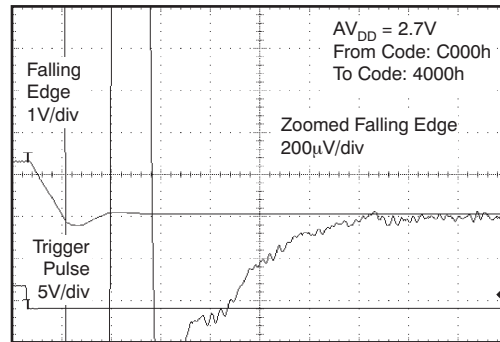
Time (2µs/div) Figure 109.
