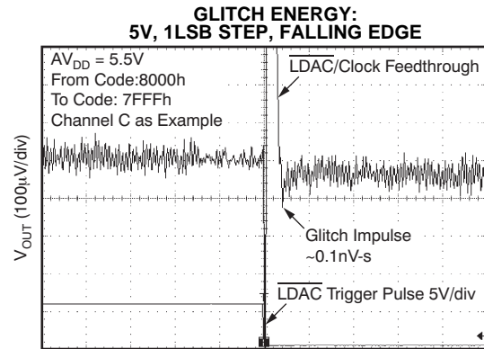
Time (5µs/div) Figure 61.
