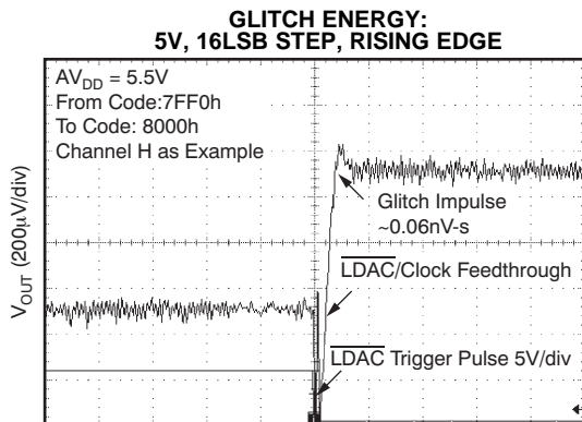
Time (5µs/div) Figure 64.
