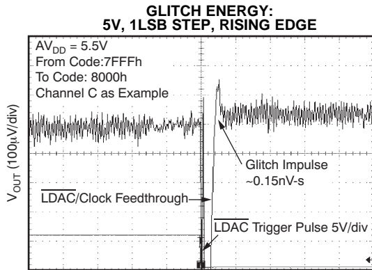
Time (5µs/div) Figure 60.
