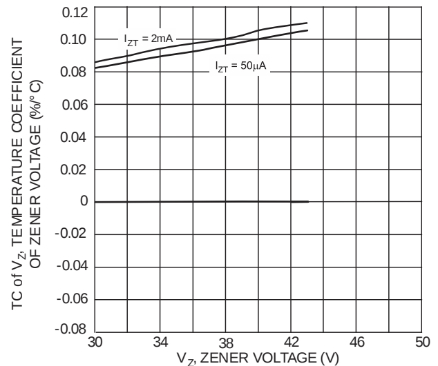
Fig. 15 Typical Temperature Coefficient of Zener Voltage vs. Zener Voltage, DDZ30DS-DDZ43S
