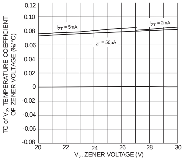
Fig. 14 Typical Temperature Coefficient of Zener Voltage vs. Zener Voltage, DDZ20CS-DDZ30DS
