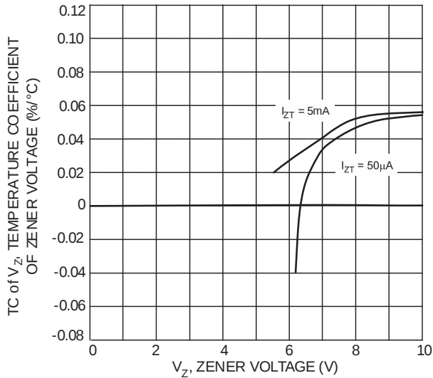
Fig. 12 Typical Temperature Coefficient of Zener Voltage vs. Zener Voltage, DDZ6V2BS-DDZ10CS
