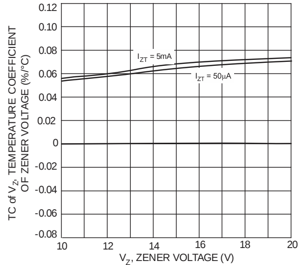
Fig. 13 Typical Temperature Coefficient of Zener Voltage vs. Zener Voltage, DDZ10CS-DDZ20CS
