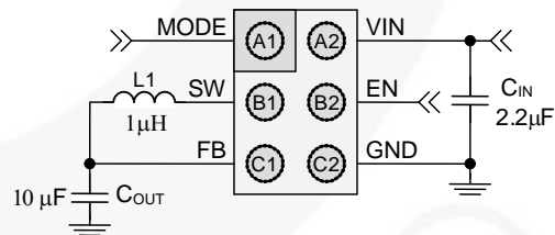
Figure 1. Typical Application
