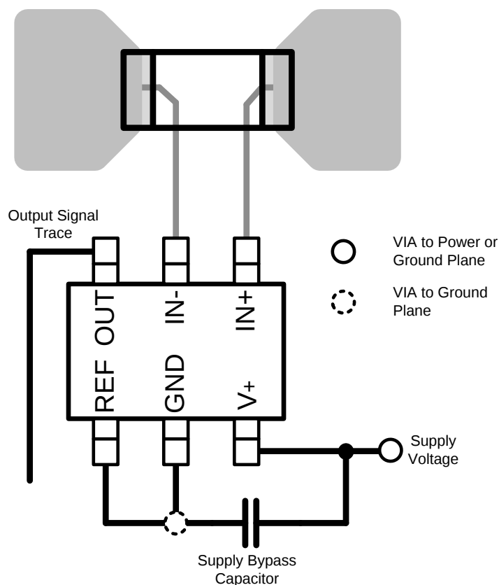
Figure 31. Recommended Layout
