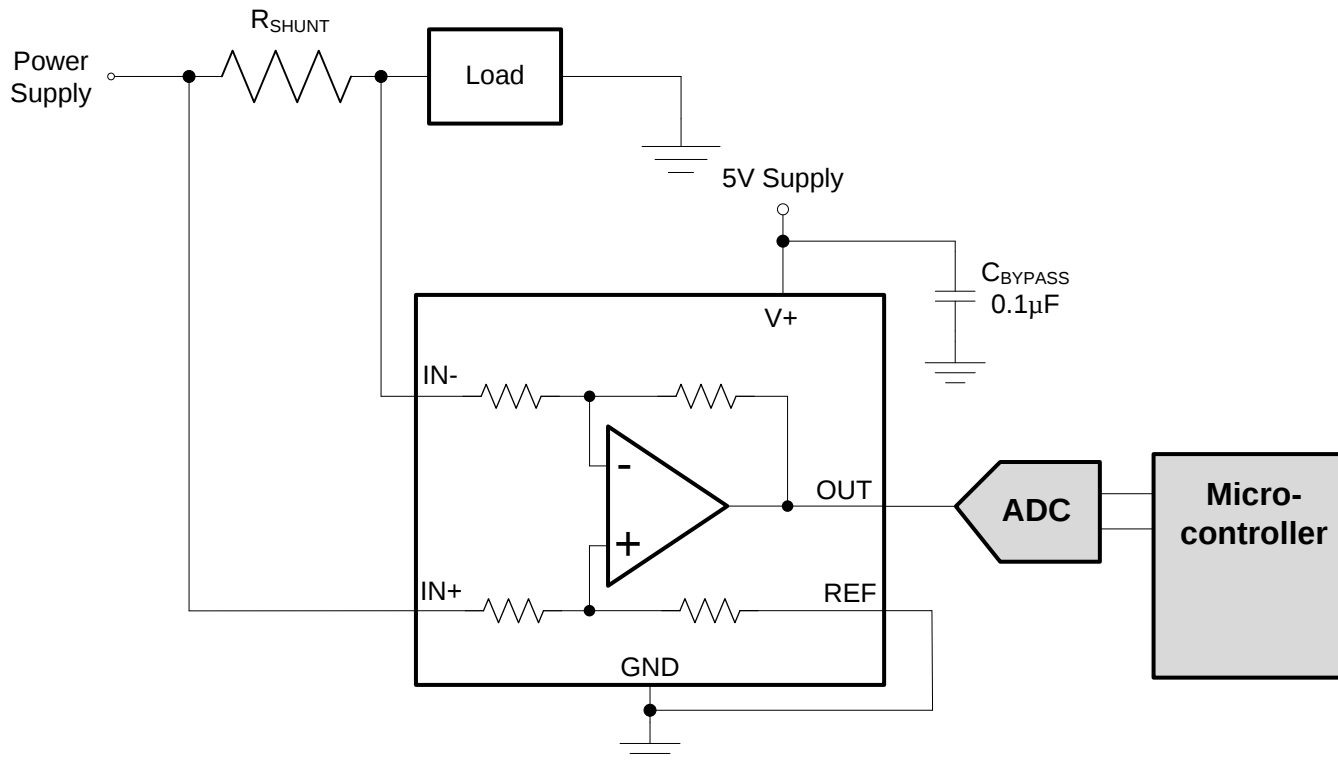
Figure 20. Typical Application
