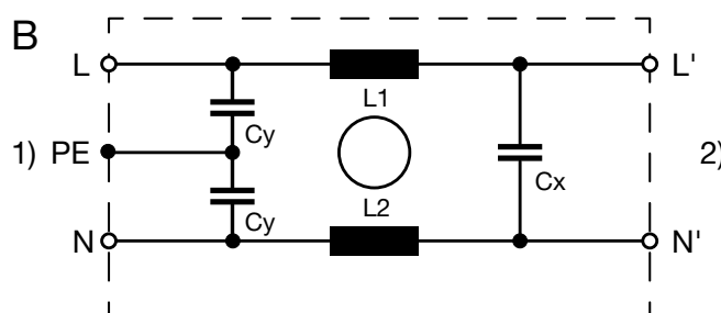
EMI filtering of equipment emissions
