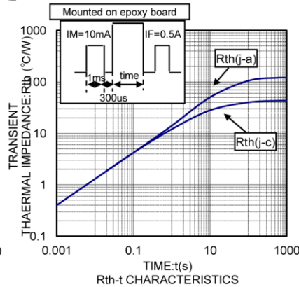
Rth-t CHARACTERISTICS
