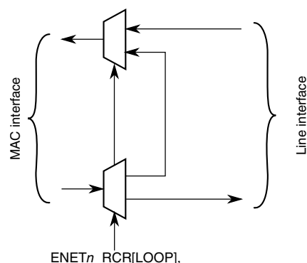
Figure 44-63. Loopback Options
