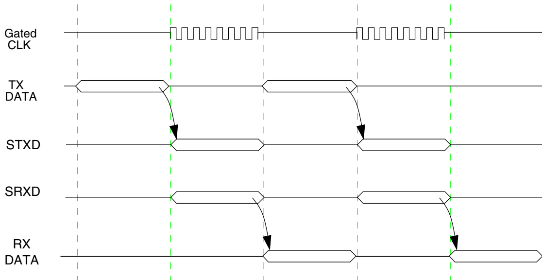
Figure 53-47. Normal mode timing - internal gated clock
