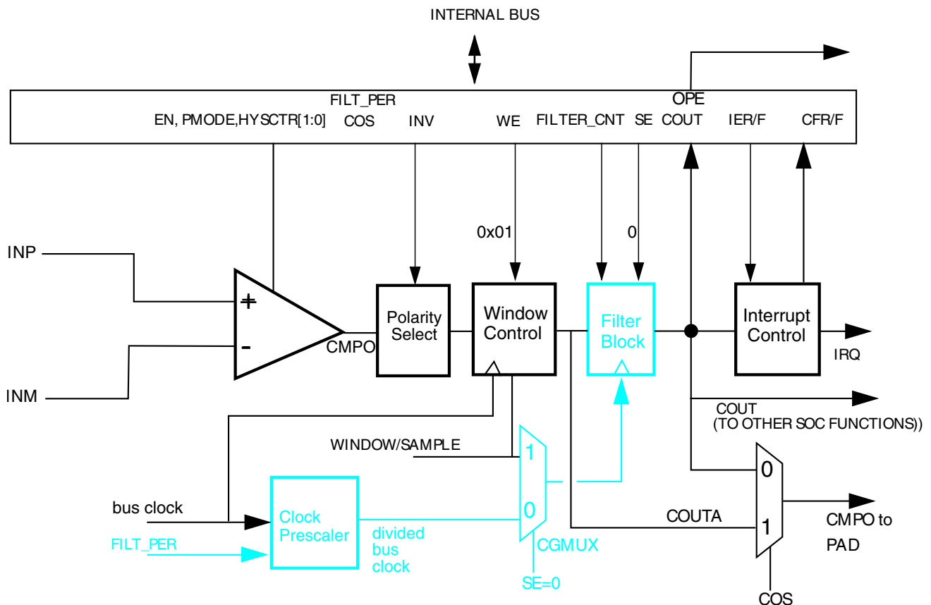
Figure 35-33. Windowed Mode
