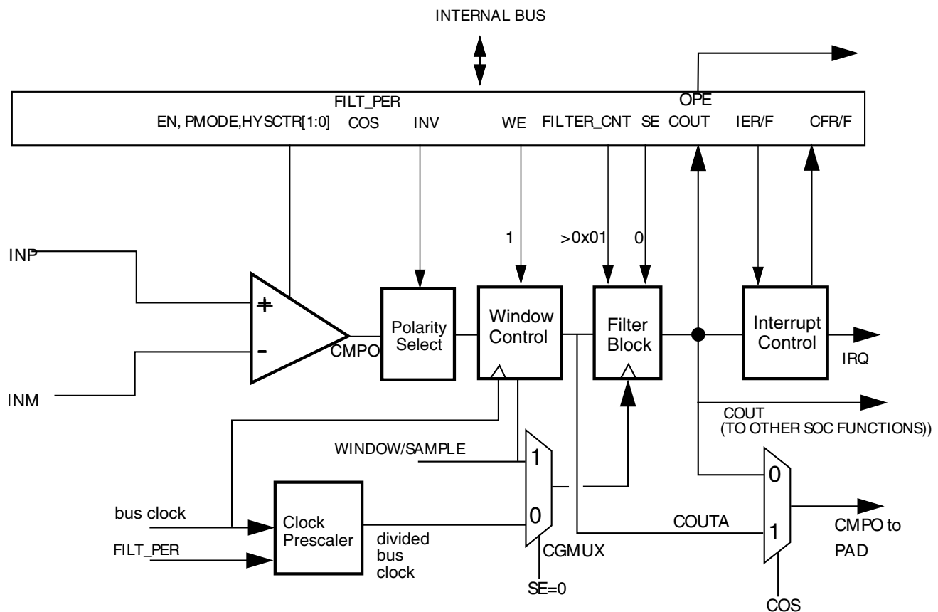
Figure 35-35. Windowed/Filtered Mode
