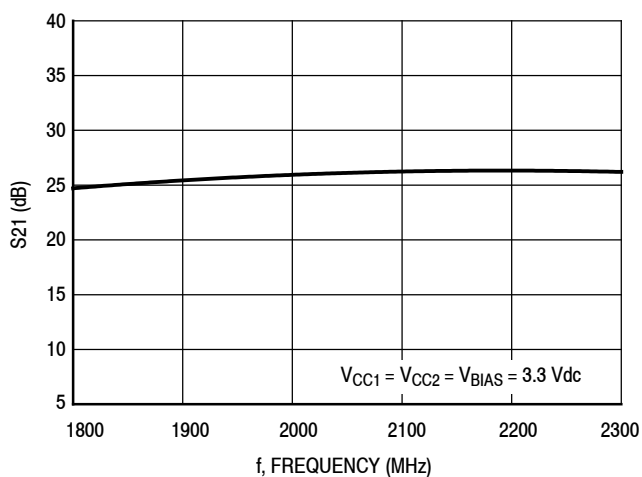
Figure 18. S21 versus Frequency
