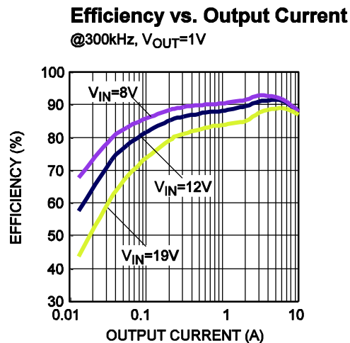
Figure 18 — Efficiency Curve
