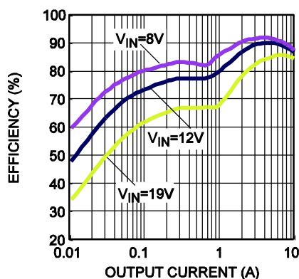
Figure 30 — Efficiency Curve
