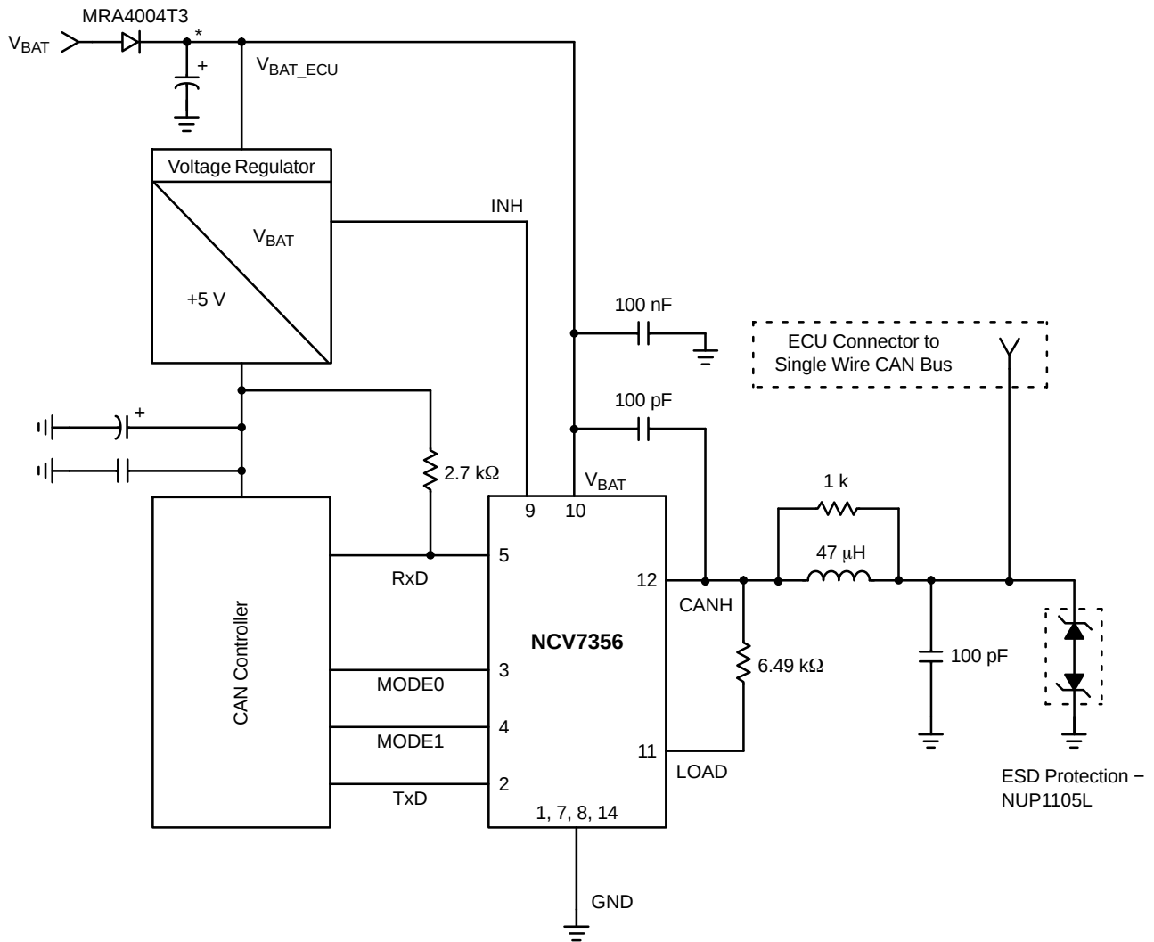
Figure 10. Application Circuitry, 14 Pin Package
