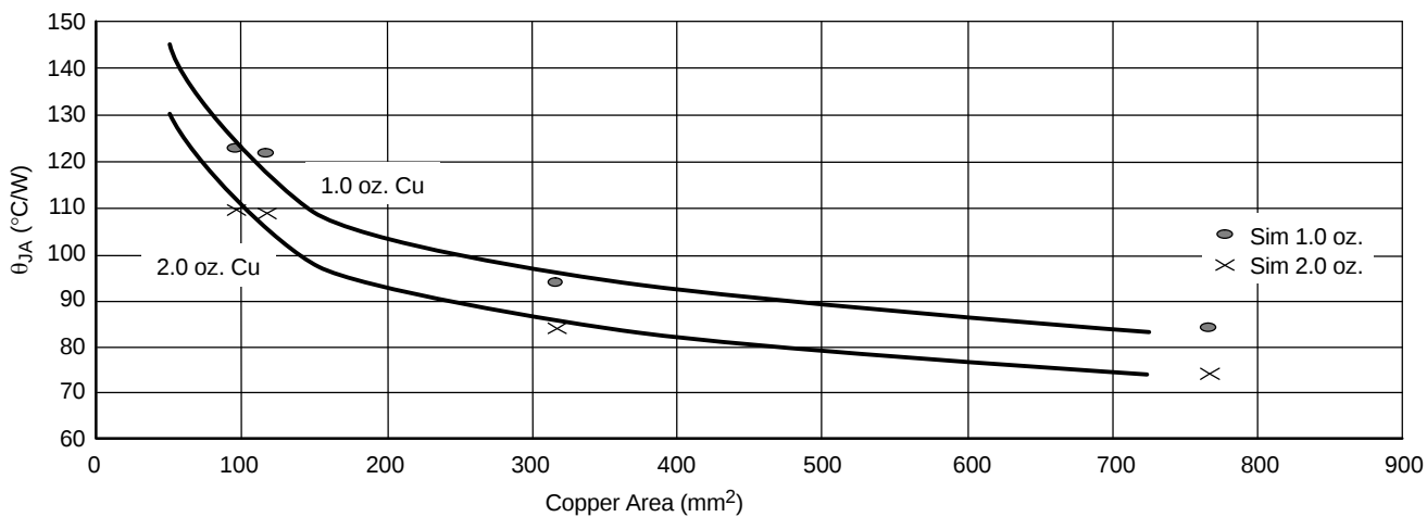
Figure 20. SOIC-14, \theta_{JA} as a Function of the Pad Copper Area Including Traces, Board Material
