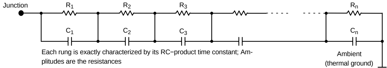
Figure 15. Non-Grounded Capacitor Thermal Ladder ("Foster" Ladder)
