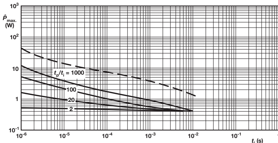
NFR25 Pulse on a regular basis; maximum permissible peak pulse power ( \hat{P}_{max} ) as a function of pulse duration ( t_i ), 15 \Omega \leq R \leq 15 \text{ k}\Omega
