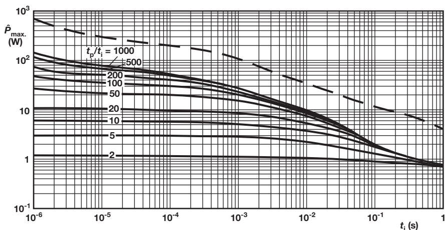
NFR25 Pulse on a regular basis; maximum permissible peak pulse power ( \hat{P}_{max} ) as a function of pulse duration ( t_i )
