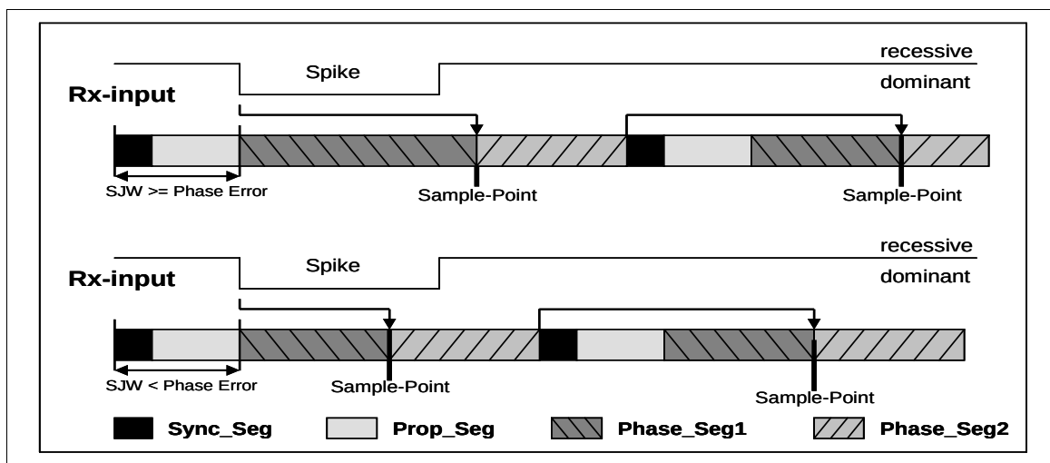
Figure 5-85 Filtering of Short Dominant Spikes
