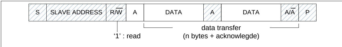
Figure 5-21 Master Reads Data from Slave
