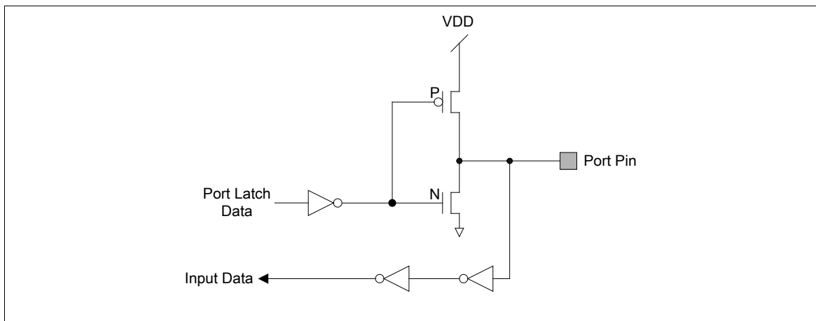
Figure 5-15 Push-Pull Output
