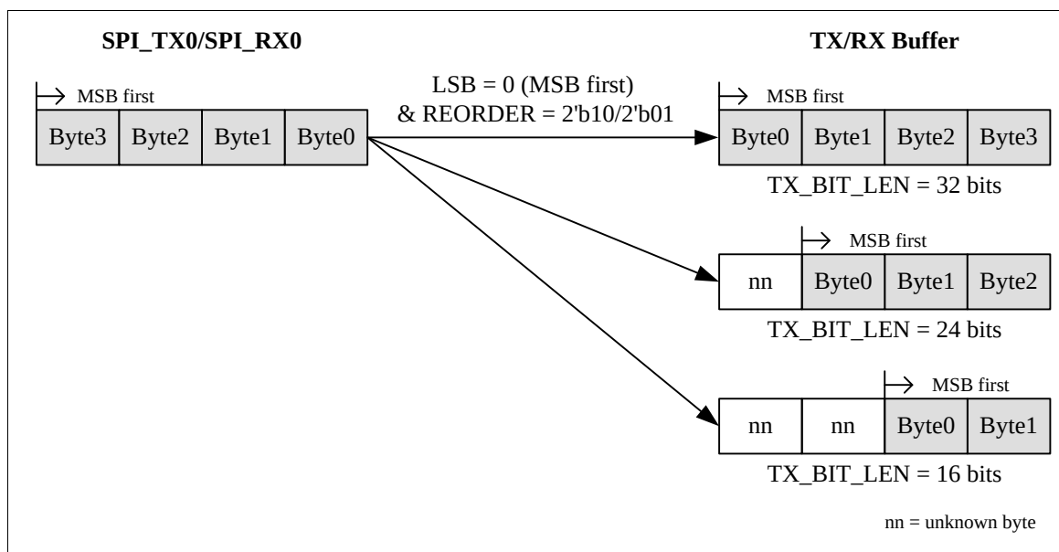
Figure 5-56 Byte Reorder
