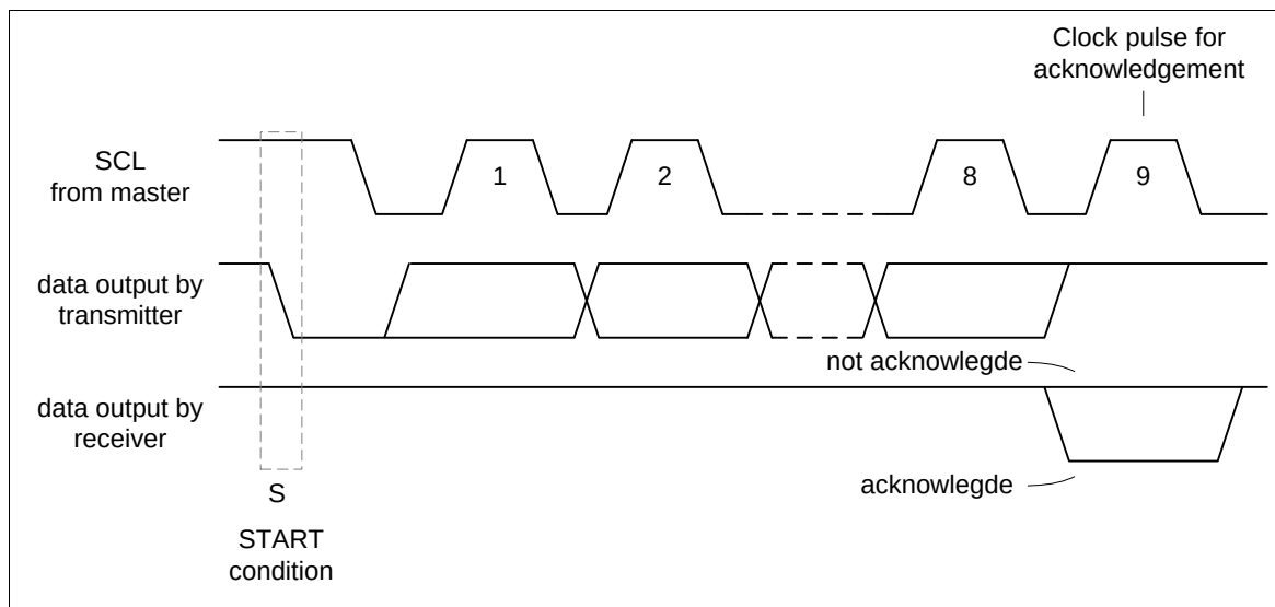
Figure 5-24 Acknowledge on I²C Bus
