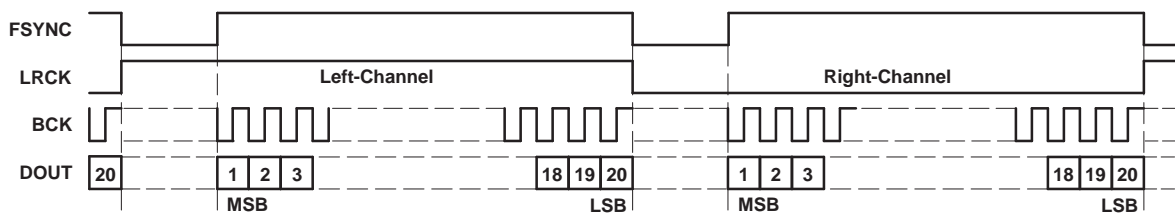
Figure 23. Audio Data Format (Master Mode: FS SYNC , LR CK , and B CK Are Outputs)
