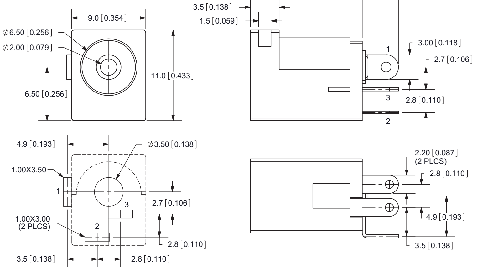
PCB LAYOUT TOP VIEW
