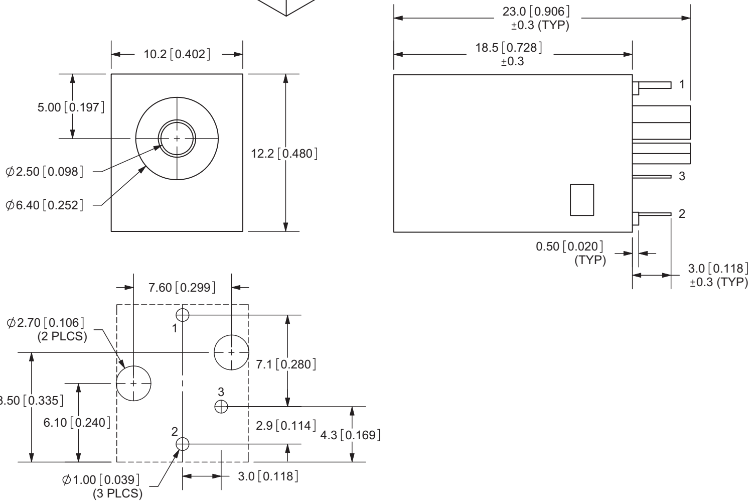
PCB LAYOUT TOP VIEW
