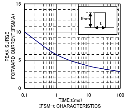
IFSM-t CHARACTERISTICS
