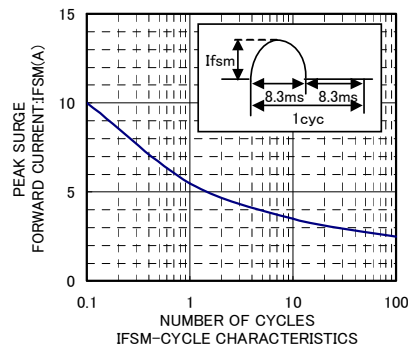
IFSM-CYCLE CHARACTERISTICS
