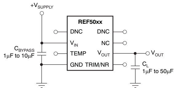
Figure 40. Basic Connections
