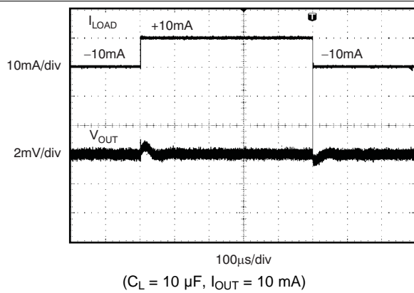
Figure 19. Load Transient
