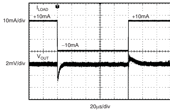
Figure 17. Load Transient ( C_L = 1\ \mu\text{F} , I_{\text{OUT}} = 10\ \text{mA} )
