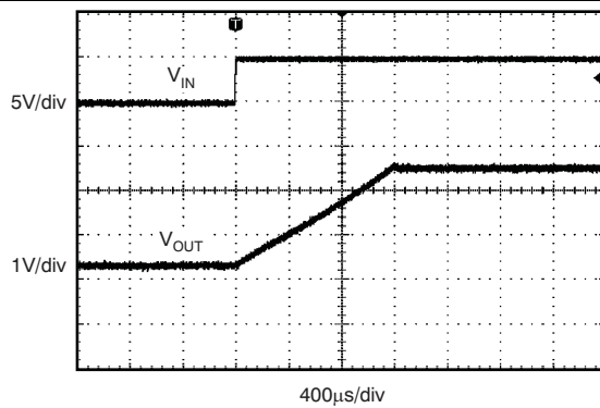
Figure 15. Start-Up (REF5025, C_L = 10\ \mu\text{F} )
