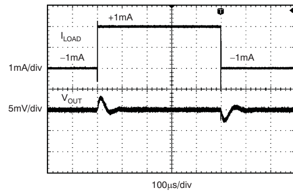
Figure 18. Load Transient ( C_L = 10\ \mu\text{F} , I_{\text{OUT}} = 1\ \text{mA} )
