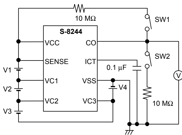
Test Circuit 2
