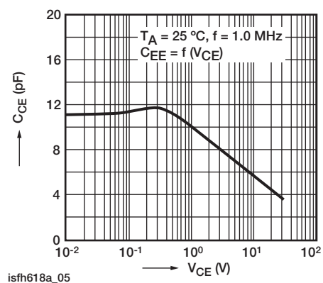
Fig. 8 - Transistor Capacitance
