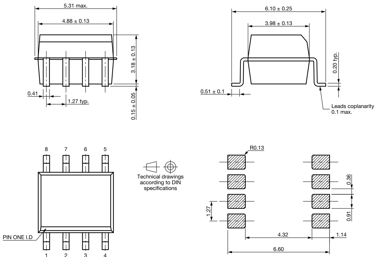
Fig. 3 - Package Drawing
