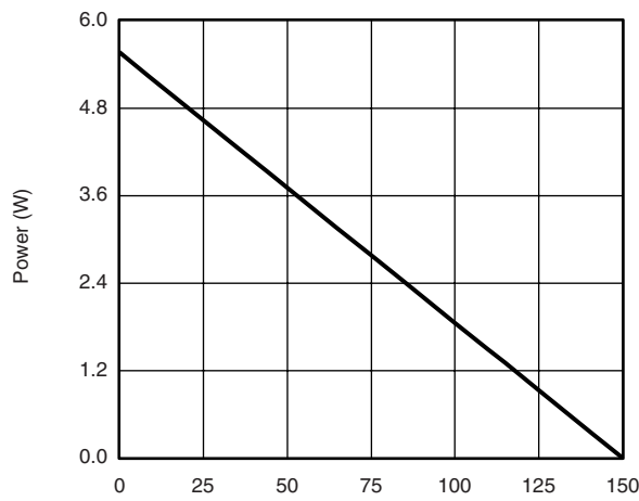
Power, Junction-to-Foot
