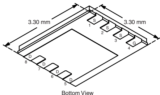
PowerPAK® 1212-8
