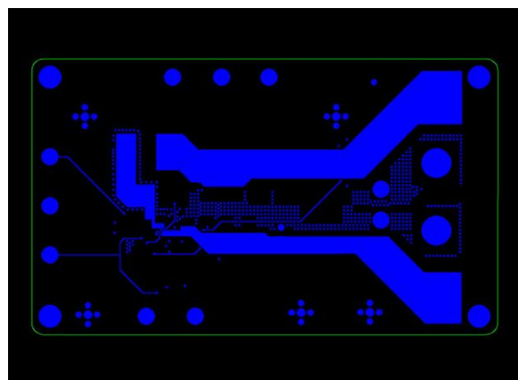
Figure 16. Mid Layer2
