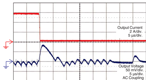
Transient Response in Power Save Mode (6 A - 0.2 A) (V_{IN} = 12\text{ V}, V_{OUT} = 1\text{ V}, F_{SW} = 500\text{ kHz at } 6\text{ A})
