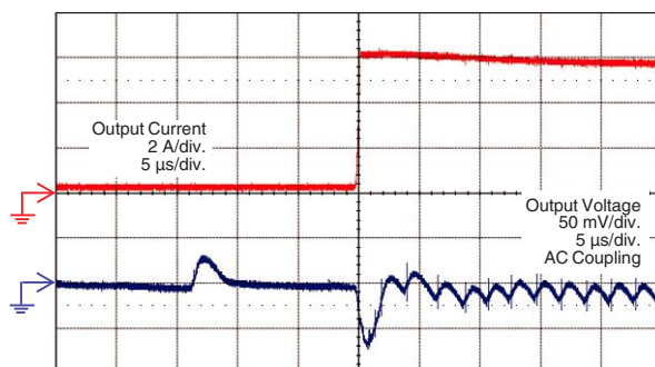
Transient Response in Power Save Mode (0.2 A - 6 A) (V_{IN} = 12\text{ V}, V_{OUT} = 1\text{ V}, F_{SW} = 500\text{ kHz at } 6\text{ A})
