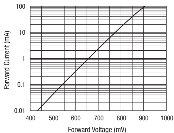
Figure 2. DC Characteristic
